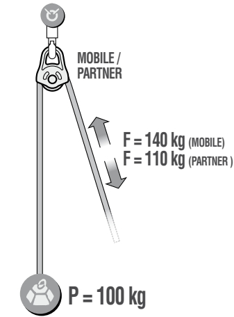
6A. Simple pulley system
