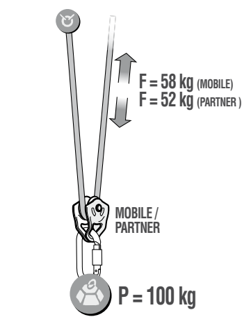
6B. 2:1 hauling system
